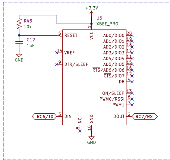
* XBEE Communication
